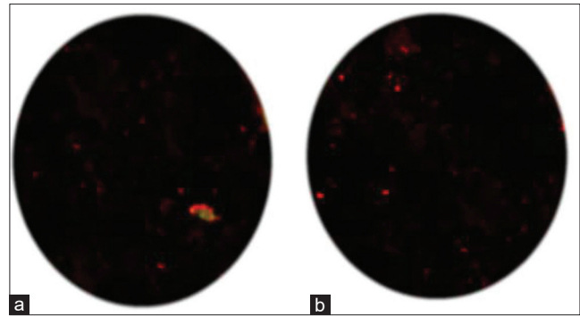
Figure 2: (a) Confocal laser scanning microscope (CLSM) images of specimens after dual fluorescence staining; Red area represents the depth of acid-etched demineralized enamel penetrated by resin infiltrant, as the dye accumulated at the progressing lesion front or beneath the resin layer. Green area represents demineralized enamel not sealed by resin infiltrant. Black area represents sound enamel and also demineralized enamel completely infiltrated with resin showed no fluorescence (b) CLSM images of specimens after dual fluorescence staining; Red area represents the depth of acid-etched demineralized enamel penetrated by resin infiltrant, as the dye accumulated at the progressing lesion front or beneath the resin layer. Green area represents demineralized enamel not sealed by resin infiltrant. Black area represents sound enamel and also demineralized enamel completely infiltrated with resin showed no fluorescence
